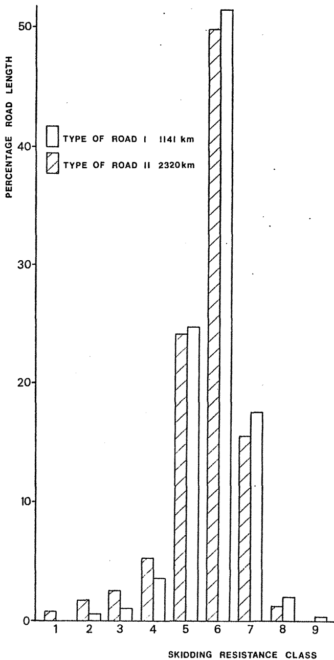
Figure 2. Total road length of the test road sectors, as a percentage of the annual total per road-type.
