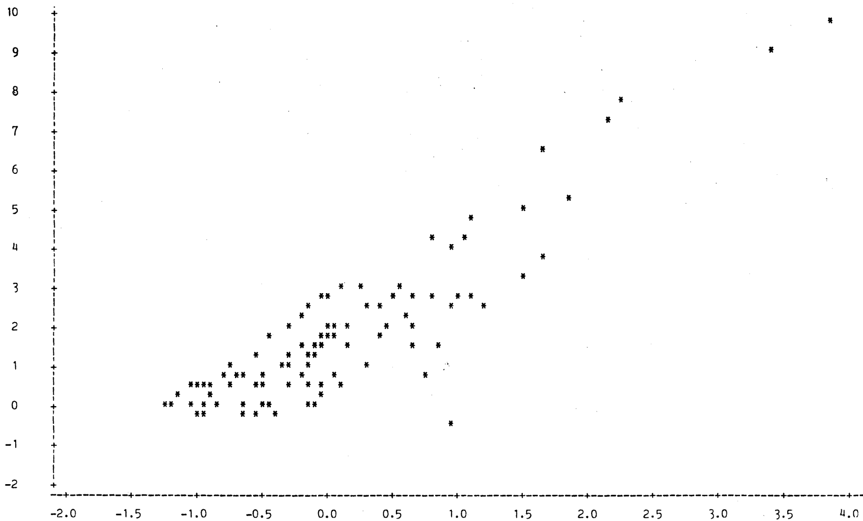
Figure 3.1. Object scores from PRINCALS analysis of all conflicts (ordinate), against those of the analysis of selected conflicts (abscissa).
